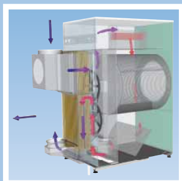
Heat recovery pipes and heat exchangers
